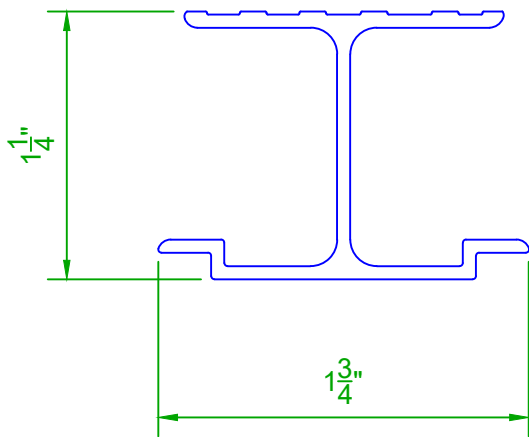
STIFFENER EXTRUSION
