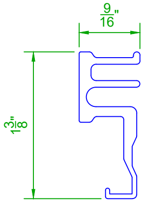
4MM FRAME EXTRUSION
