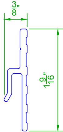
FIELD CLIP EXTRUSION
