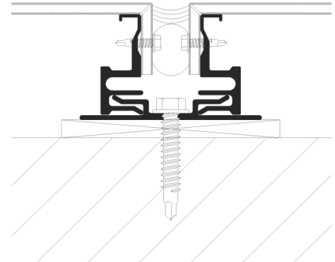
A2000 Series Wet Seal System
