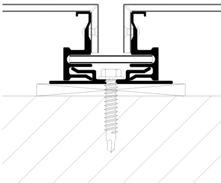
A1000 Series D-B/V System
