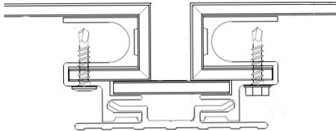
A1000NF Series D-B/V System
