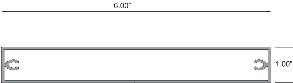
1" x 6" Batten #1.18 LBS/Inft
