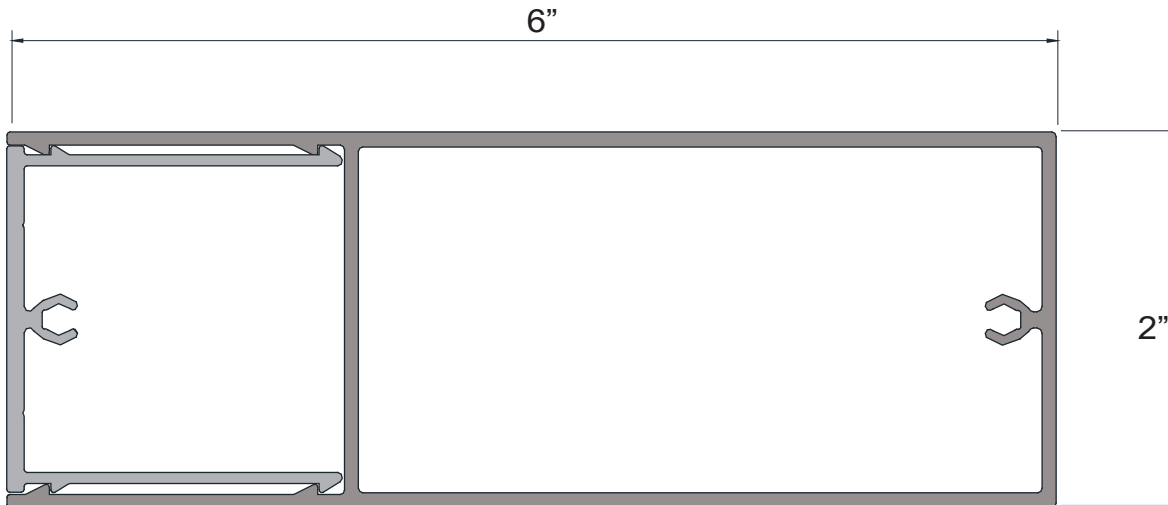
2"x 6" Vertical Interlocking Batten
