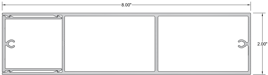
2" X 8" Batten Assembly
