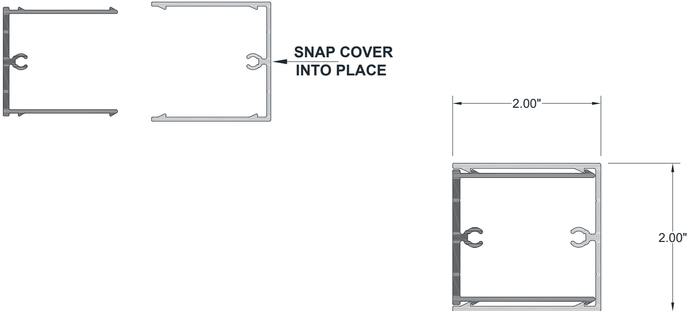
2" x 2" BATTEN ASSEMBLY
