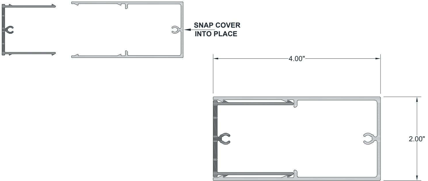
2" x 4" BATTEN ASSEMBLY
