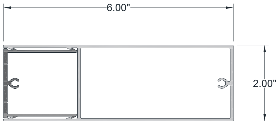
2" x 6" BATTEN ASSEMBLY
