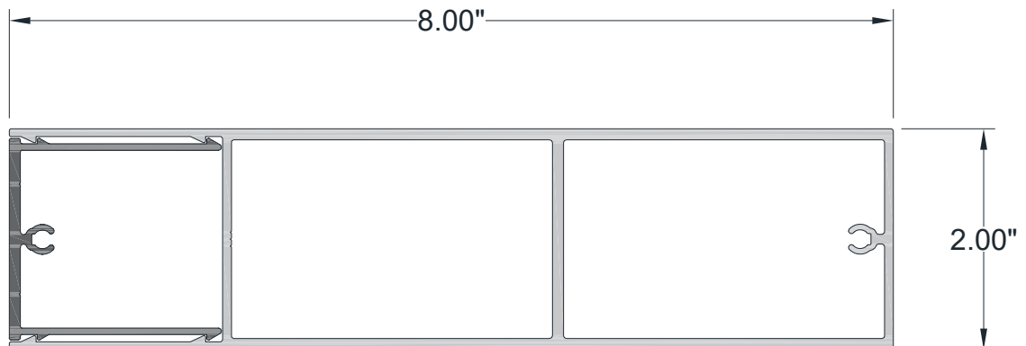
2" x 8" BATTEN ASSEMBLY
