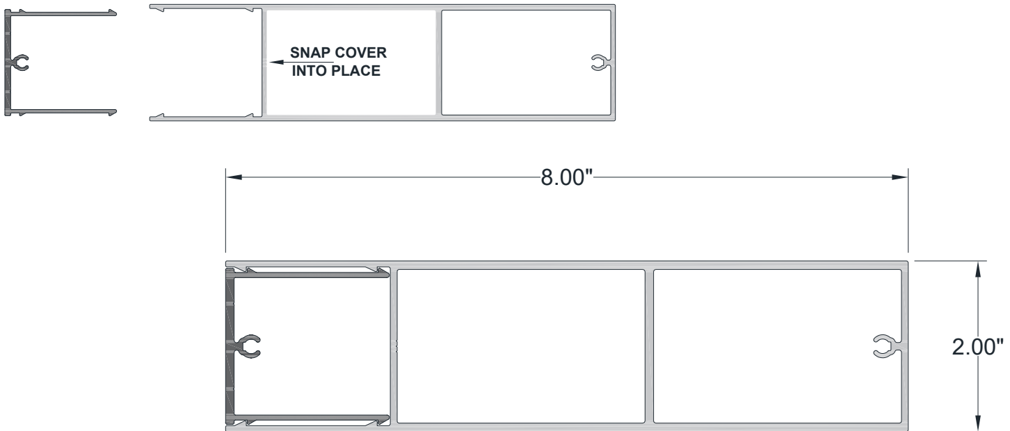
2" x 8" BATTEN ASSEMBLY
