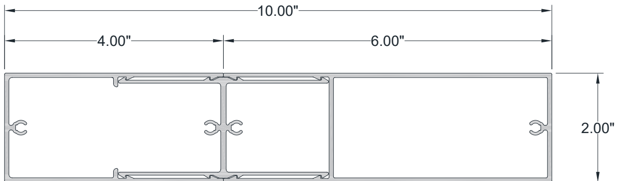
2" x 10" BATTEN ASSEMBLY
