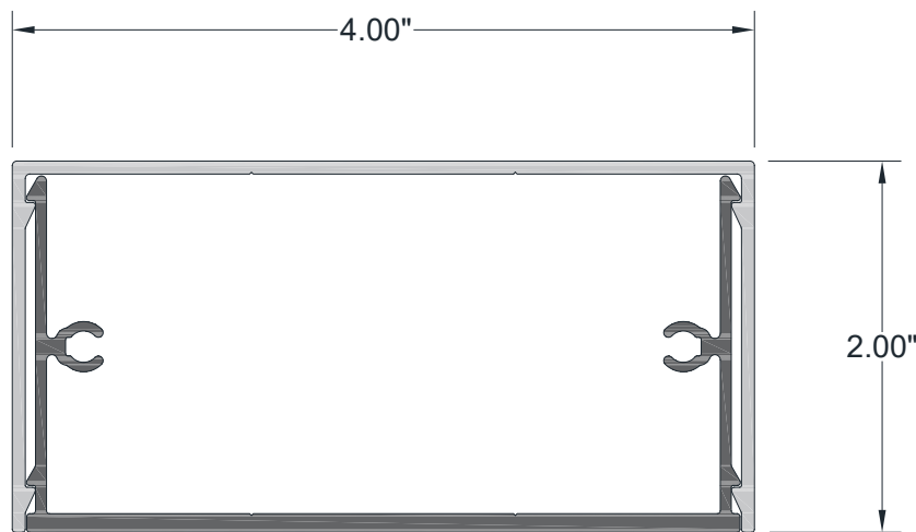
4" x 2" BATTEN ASSEMBLY
