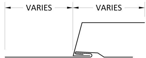
Panel engagement detail
