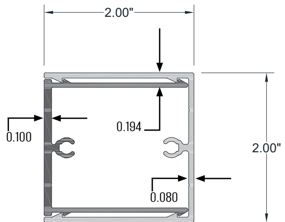
2" x 2" BATTEN ASSEMBLY
