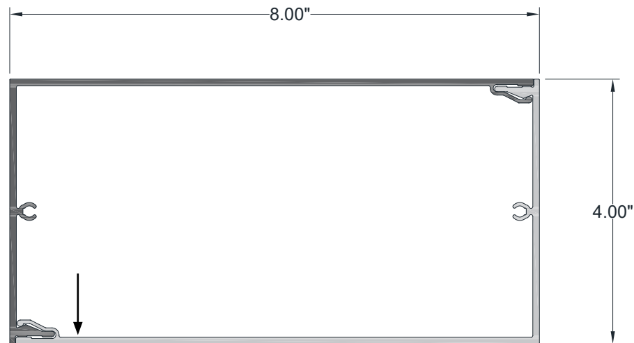
4" x 8" BATTEN L-CONNECT ASSEMBLY
