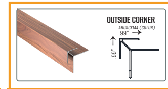
Outside Corner
