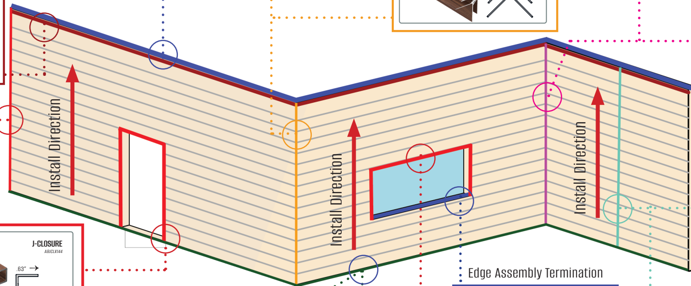
Option 2 Inside Corner Assembly
