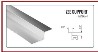
Zee Support
