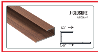
J-Closure
