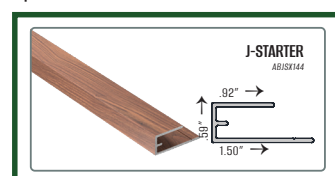
Option 1 J-Starter
