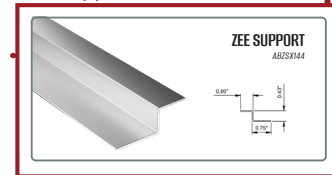
Zee Support
