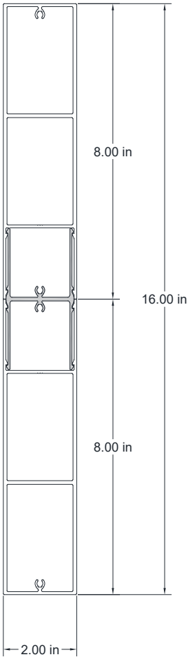
i) 2x16 snap fit assembly
