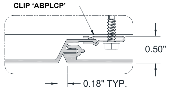
PLANK ENGAGEMENT
