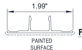
JOINT BASE
