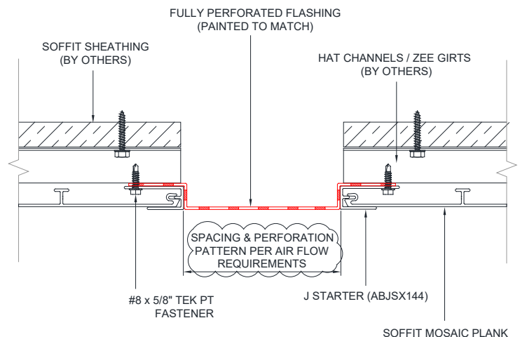
Typical Venting
