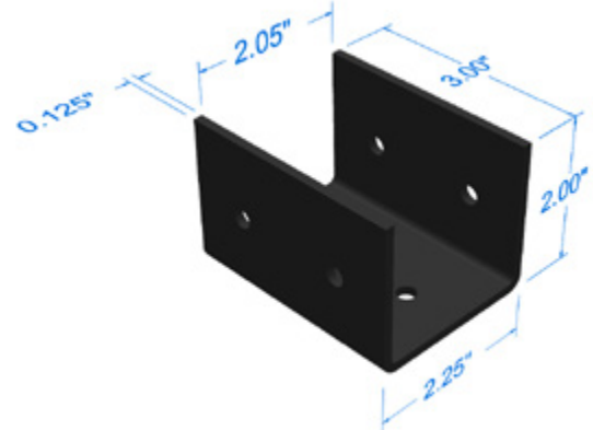
2" U BRACKET
