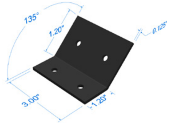
ANGLE BRACKET
