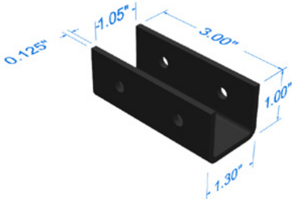
1" U BRACKET
